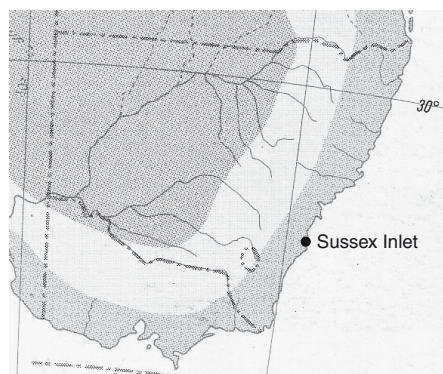
Figure 1. National bitou bush Southern Containment Line at Sussex Inlet, approximately 200 km south of Sydney.
